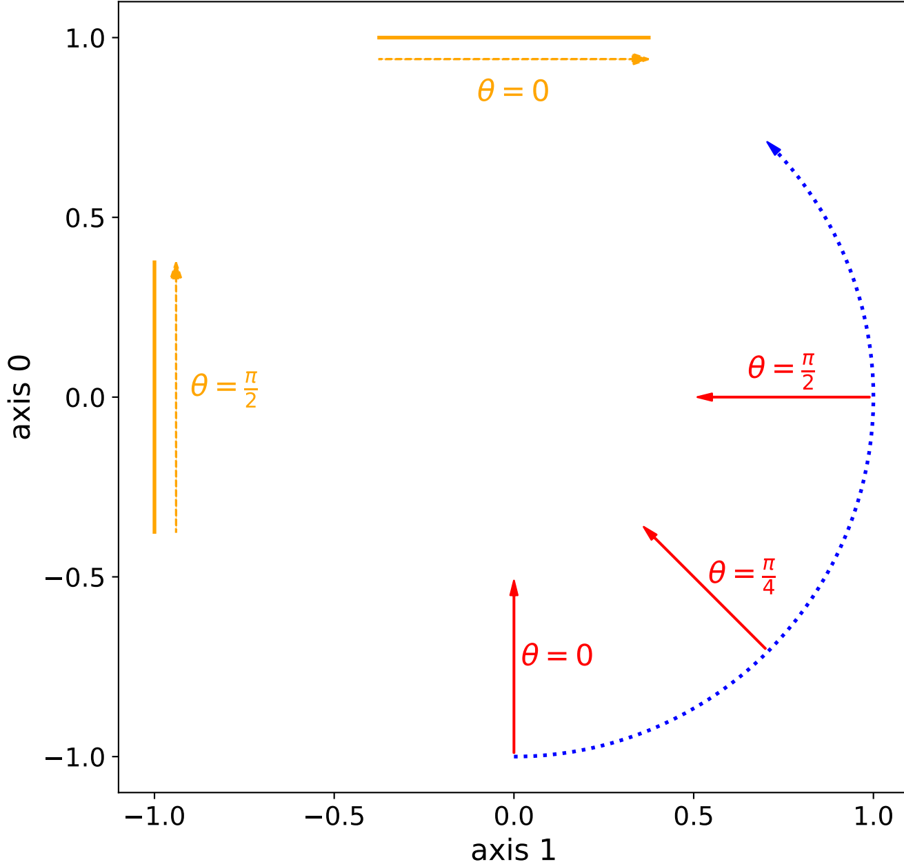
astra
